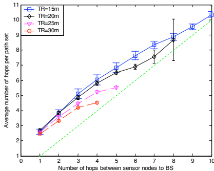
Fig. 7. The quality of the alternate paths
