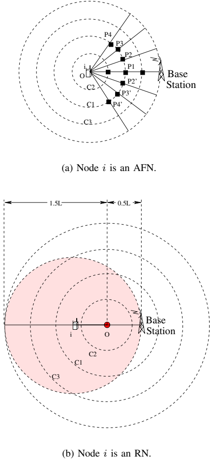
Fig. 4. INDS step in the SPINDS algorithm.
